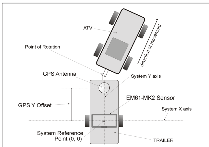
Figure 3.2: Geometry of the EM61-MK2 sensor and GPS antenna during towing
