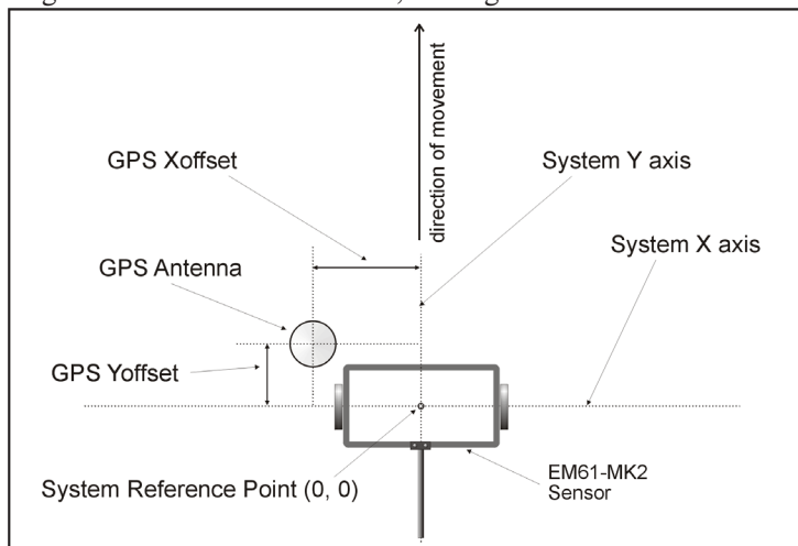
Figure 3.1: The EM61-MK2 and GPS antenna geometry
