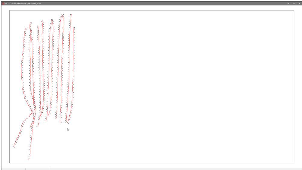
Figure 3.30: Two dimensional layout of stations taken with the Geonics EM61-MK2. The GPS X and Y offsets: GPS X Offset = 0.4 m and GPS Y Offset = 0.02
