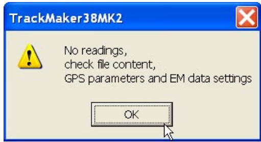
Figure 3.12: Warning window
