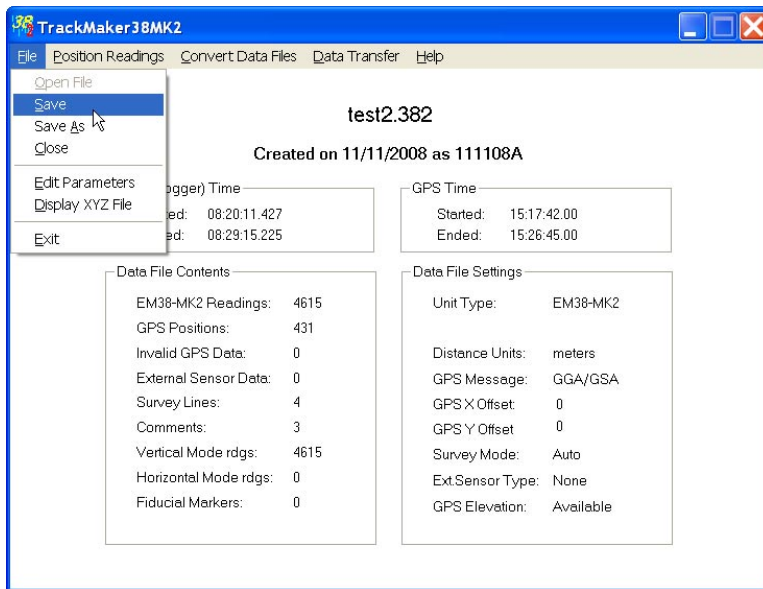
Figure 2.5: TrackMaker38MK2 Main Screen with item Save enabled after not original file was loaded
