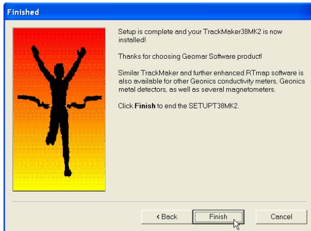
Figure 1.9: Finished window
