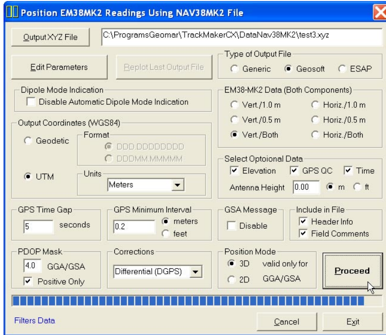
Figure 3.9: Position EM38-MK2 Readings Using NAV38MK2 File window during creating XYZ file
